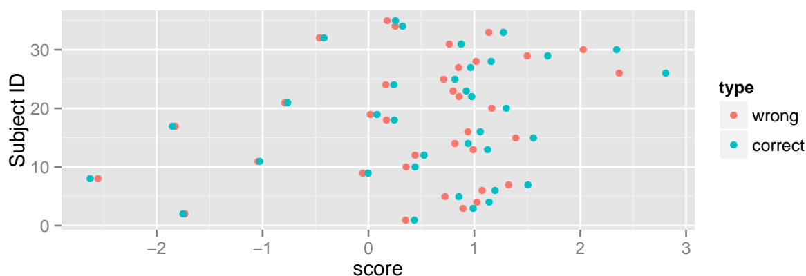
Figure 4.6: EAP scores with a standard Normal latent distribution (wrong) and estimated Normal distribution (correct).
